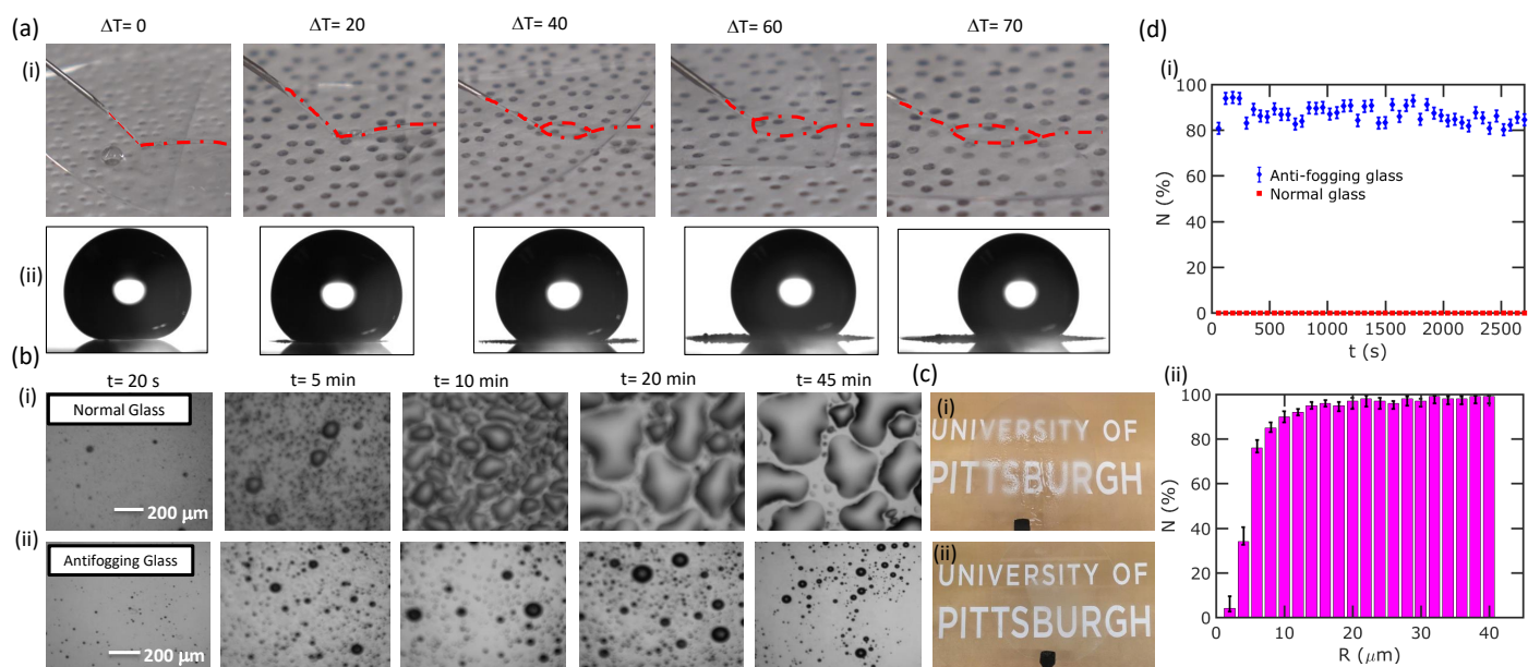
Fig. 5 (a) (i) shows water jet behaviour as a function of temperature \Delta T . (a)(ii) shows the water contact angle at different \Delta T on antifogging glass. Condensation versus time optical images of (b)(i) normal glass and (b) (ii) antifogging glass. (c) shows optical image of (i) normal and (ii) antifogging glass after 45 min of condensation. (d) (i) plot of percentage of jumping droplets after coalescences versus time. (c)(ii) Relationship of percentage of coalescences droplets jumping and radius of the droplet at the moment of jumping.
