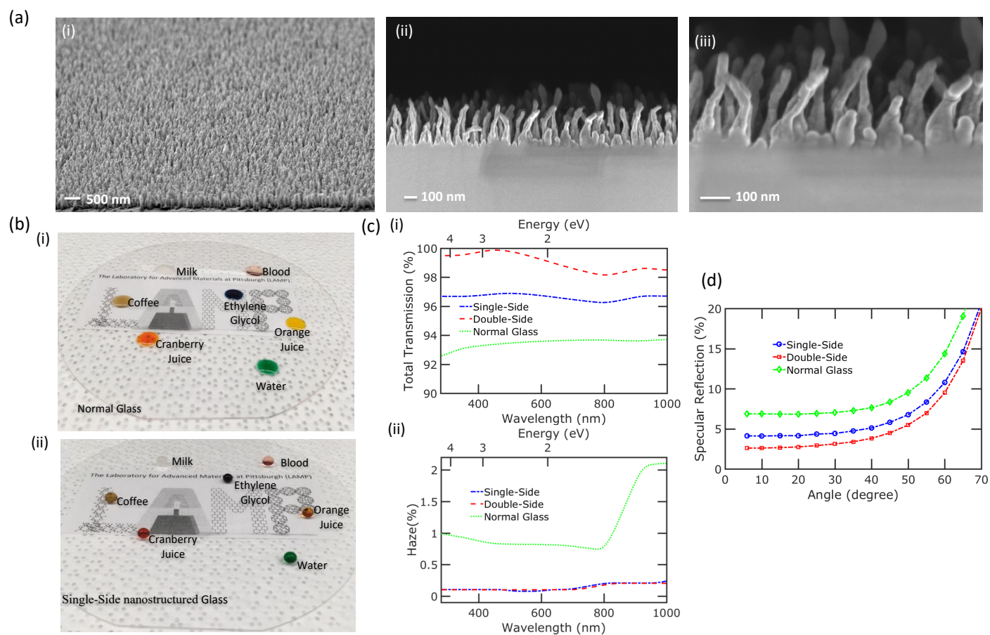
Fig. 4 (a) shows (i) 20° tilted, (ii) and (iii) cross sectional SEM images of fabricated glass with different magnifications. (b) shows the droplet of different liquids on (i) normal and (ii) our superomniphobic glass. (c) (i) show transmission and (ii) haze plots as a function of wavelength for bare, single side and double side etched glass (d) Angle-resolved spectra for reflection at 550 nm wavelength for bare, single side and double side etched glass.
