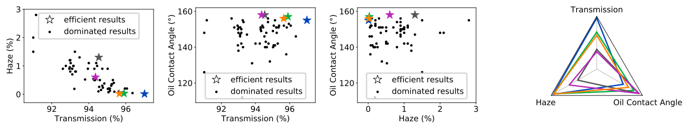
Fig. 3 Depictions of the experimental design driven by our Bayesian optimization methodology. left : Three 2D feasible region plots of the three objectives under consideration. right : Radar plot of the 5 viable efficient outcomes identified during the parameter search (plot qualitatively exaggerated to account for the different scales of the three objectives).
