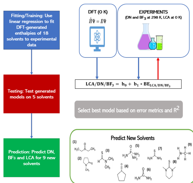
Fig. 1 Work flow showing how linear models describing the affinity metrics are constructed to allow predictions of these metrics for nine solvents: 1) DESO 2) NMPT 3) DMTF 4) THTO 5) PA 6) Urea 7) Thiourea 8) DMDT and 9) Methylamine. See Table 1 for the full names of the solvents. The lefthand column provides the workflow of the procedure. The righthand column provides more details on these steps. BE refers to the binding enthalpy between the solvent and the relevant Lewis acid.
