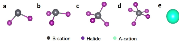
Fig. 3 Schematic of the perovskite acids explored: a) BX_2 salt complexes e.g. PbX_2 , SnX_2 and GeX_2 b) BX_3 salt complexes e.g. BiX_3 and SbX_3 c) BX_4 salt complexes e.g. SnX_4 d) BX_5 salt complexes e.g. SbX_5 (where X = Cl^- , Br^- , and I^- ) and e) A-site cations e.g. Na^+ , K^+ , Rb^+ and Cs^+ . Color code as in inset.
