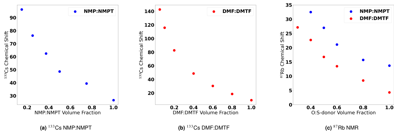
Fig. 7 ^{133}Cs NMR chemical shifts as a function of the ratio of O-donor solvent to S-donor solvent in solution showing (a) results for various mixtures of NMP and NMPT and (b) results for mixtures of DMF and DMTF. c) ^{87}Rb NMR chemical shifts as a function of the ratio of O-donor solvent to S-donor solvent in solution for mixtures of NMP:NMPT and DMF:DMTF.
