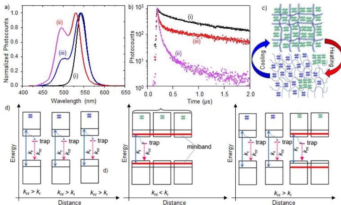
Fig. 3. a) PL spectra ( \lambda_{\text{ex}} = 400 nm) and b) PL decays ( \lambda_{\text{ex}} = 405 nm) of a dried (4.5 h) PQD-PBD film. (a) The spectra at (i) 296 K before heating, (ii) 323 K, and (iii) 296 K after heating and cooling. (b) The decay (i) corresponds to the PL spectrum (i) in 'a', and the decay (ii) and (iii) correspond to the photons in the 440-515 nm range, and 515-570 nm range, respectively for the PL spectrum (ii) in 'a'. c) A scheme of PQD assembly formation and dissociation during drying and the heating-cooling cycle. (d) A scheme of energy states, photoexcitation, and relaxation in PQDs before and after assembly formation, heating, and cooling ( k_{\text{nr}} : nonradiative recombination rate and k_r : radiative recombination rate).
