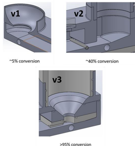
Figure 10: Section Views of Three Iterations of the Melting Zone Design of the Top Plate and Corresponding Maximum Conversions that were Achieved.
