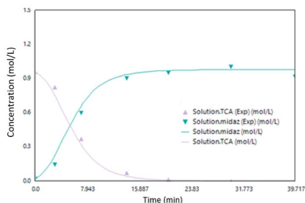
Figure 3: Kinetic Model Validation Experiment for the Synthesis of Midazolam at 230 °C with 5.8 equiv. PTSA (midaz = midazolam).
