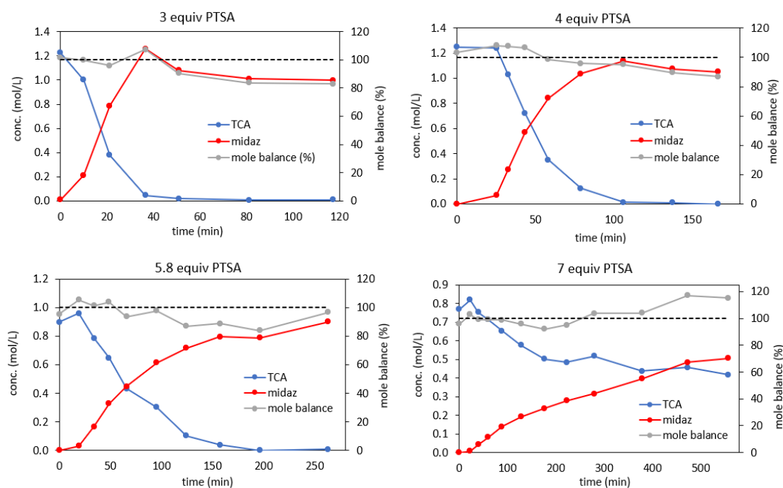
Figure 1: Concentration profiles for small scale batch syntheses of midazolam from TCA using different equivalents of PTSA. All reactions were performed at 200 °C (midaz = midazolam). The lines are for illustrative purposes and are not intended to imply a modeled system. Mole balance is calculated by dividing the sum of the midazolam and TCA concentrations by the initial TCA concentration.
