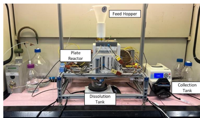
Figure 13: Plate Reactor Equipment Train for the Production Campaign.
