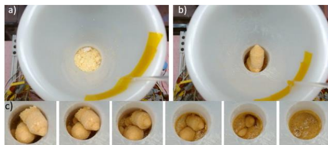
Figure 11: a) Overhead view of the plate reactor feed hopper with loose powder. b) Feed hopper with powder plugs formed in conical vials. c) Time-lapse view of the powder plugs traveling down the feed hopper and melting.
