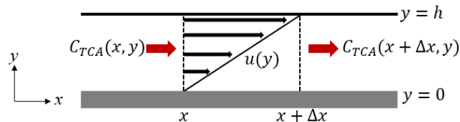
Figure 5: Diagram of the Melt Flow Model Used to Derive the Material Balance in the Plate Reactor.
