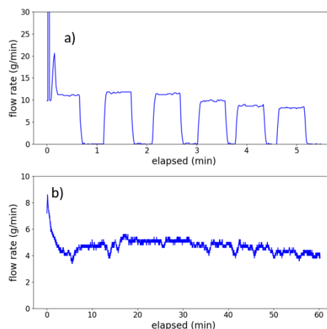
Figure 7: Flow profiles for a) unoptimized and b) optimized plate outlets. Water was fed at a constant rate to the plates via an addition funnel and the flow rate exiting the plates was measured via a scale.
