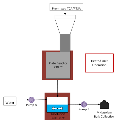
Figure 12: Process Flow Diagram of the Plate Reactor and Continuous Dissolution.
