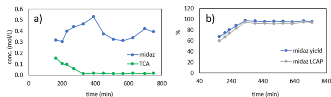
Figure 14: Results of 13-hour Production Campaign. a) molar concentration of TCA and midazolam in dissolution outlet b) instantaneous yield and LCAP of midazolam in dissolution outlet. LCAP = liquid chromatography area percent. Midaz = midazolam.
