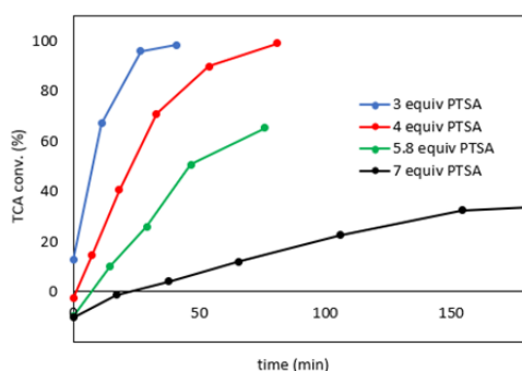
Figure 2: Effect of PTSA equivalents on TCA conversion at 200 °C. The lines are for illustrative purposes and are not intended to imply a modeled system.
