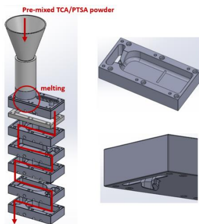
Figure 4: Initial Computer-Aided Design (CAD) Design and Operating Principle of the Plate Reactor.
