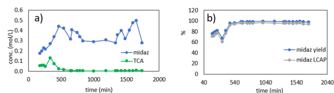
Figure 15: Results of 28-hour Production Campaign. a) molar concentration of TCA and midazolam in dissolution outlet b) instantaneous yield and LCAP of midazolam in dissolution outlet. LCAP = liquid chromatography area percent. Midaz = midazolam.
