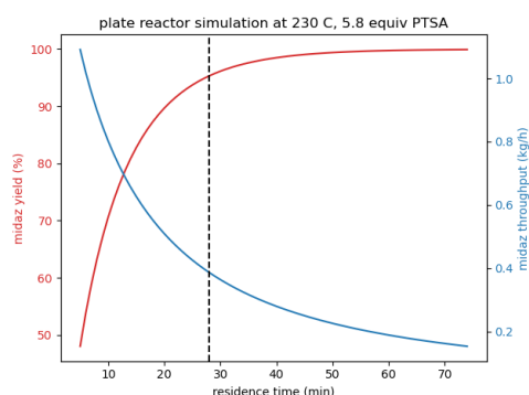
Figure 6: Plate Reactor Simulation Results at 230 °C with 5.8 Equiv. PTSA. Midaz = midazolam.
