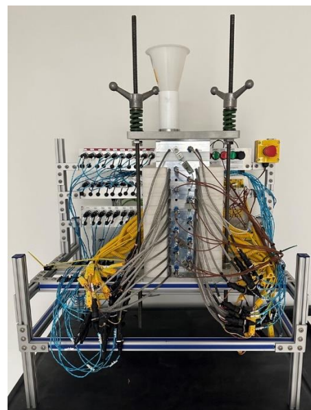
Figure 16: Scaled-Up 2 nd Generation Plate Reactor.
