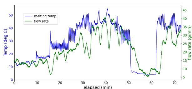
Figure 9: Overlay of the Temperature of the Top Plate and Water Flow Rate at the Outlet of the Plate Reactor.
