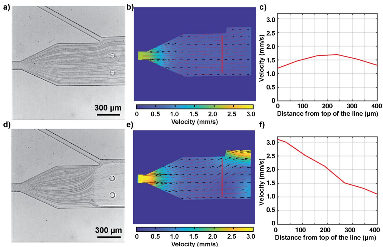
Figure 2. Fluid flow reconfiguration upon creation of the temporary hydrogel wall. (a,d) Flow pathlines before (a) and after (d) gel polymerization visualized by combining high-speed images of tracer particle flow. (b,e) Flow velocity vector streamlines and spatial profiles before (b) and after (e) gel polymerization. (c,f) Flow velocity profile along the vertical line in panel b and e, respectively.
