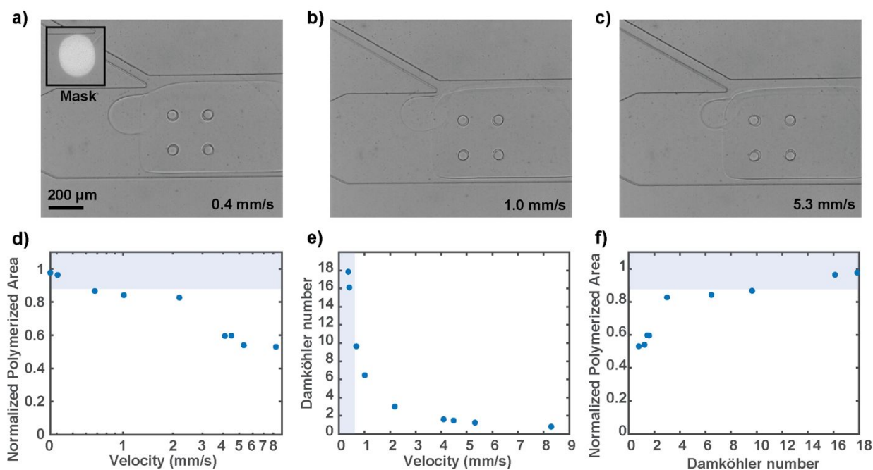
Figure 4. Characterization of the extent of gel polymerization in a flowing prepolymer of different velocities. (a,b,c) Qualitative size comparison of circular hydrogel polymerized under different flow rates. (d) Flow
