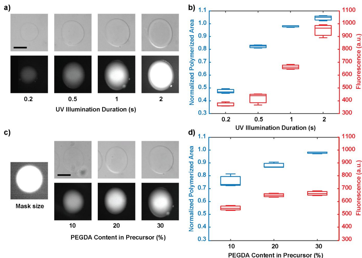
Figure 3. Optimization and characterization of the gel polymerization in relation to UV dosage and crosslinker content. (a) Visual comparison of hydrogel size and fluorescence intensity by UV illumination duration. The fluorescence intensity indicates the crosslinking density of the hydrogel. (b) The effect of UV illumination duration on the cross-sectional area of polymerization (left-axis) and the polymerization density indicated by signal of conjugated fluorophore (right-axis). The area of the polymerized gel is normalized by the mask area. (c) Visual comparison of hydrogel size and fluorescence intensity by PEGDA content in precursor. (d) The effect of percentage of PEGDA in the prepolymer solution on the cross-sectional area of polymerization (left-axis) and the polymerization density indicated by signal of crosslinked fluorophore (right-axis). For each box plot in panel b and d, the central mark indicates the median, and the outline indicates the lower and upper quartiles. For each box plot, the center line indicates the median, and the bottom and top edges indicate the 25th and 75th percentiles, respectively. The whiskers indicate the most extreme data points that are not outliers. Scale bar: 100 \mu\text{m} .
