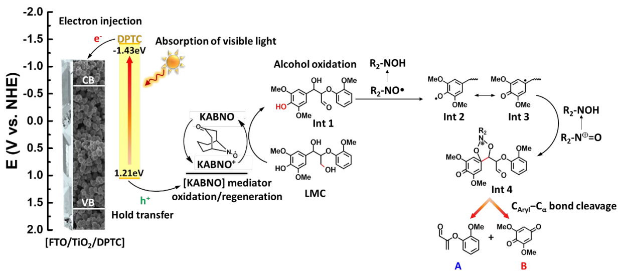
Figure 6. Proposed mechanism for oxidative C–C bond cleavage to give products A and B in the DSPEC system by using the FTO/TiO 2 /DPTC photoanode and KABNO (R 2 NO • ) in the presence of LMC .
