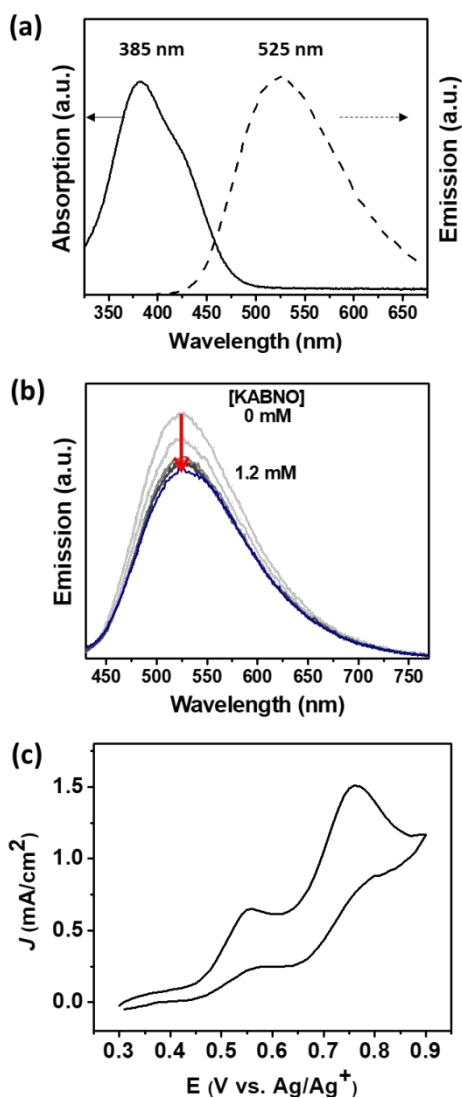
Figure 2. (a) UV-vis absorption (solid) and emission (dash) spectra of DPTC in acetonitrile. Emission spectrum was obtained with excitation at \lambda_{\text{ex}} = 380 nm. (b) Emission quenching for DPTC with KABNO (conc. = 0 – 1.2 mM). (c) CV of KABNO and LMC in 0.1 M TBAPF 6 acetonitrile solution. The experiment was performed using a glassy carbon working electrode, Pt counter electrode, and Ag/Ag + reference electrode in the dark.
