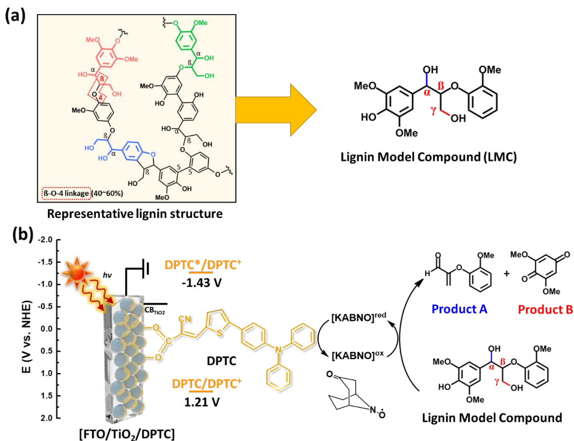
Figure 1. (a) Schematic representative structure of real lignin (left) and a dimeric lignin model compound (LMC) containing abundant aryl ether linkage (right), and (b) illustration of DPTC anchored on mesoporous structured TiO 2 for solar light-driven oxidative cleavage of LMC in combination with a bicyclic nitroxyl mediator, 9-azabicyclo[3,3,1]nonan-3-one-9-oxyl (KABNO).
