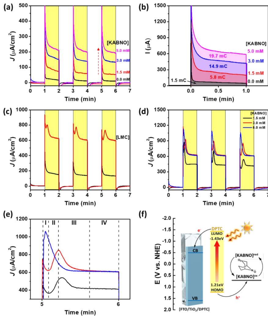
Figure 4. (a) Photocurrent-time trace of FTO/TiO 2 /DPTC (black) with different concentration of KABNO (red: 1.5 mM, blue: 3.0 mM, and pink: 5.0 mM). (b) Chronoamperograms of the FTO/TiO 2 /DPTC electrode in the presence of increasing concentration of KABNO from under illumination from time 0 to 1 min. Photocurrent-time trace of FTO/TiO 2 /DPTC (c) with 3 mM KABNO (black) and the mixture of 3 mM KABNO and LMC (red), (d) with different concentration of KABNO (black: 1.5 mM, red: 3.0 mM, and blue: 6.0 mM) at 3 mM LMC , and (e) the photocurrent densities with the period of between 5 and 6 min. (f) Energy diagram of the mesoporous TiO 2 , DPTC , and KABNO components of system. CB and VB indicate the conduction band and valence band potential of TiO 2 , respectively. All photocurrent-time trace experiments performed in 0.1 M TBAPF 6 acetonitrile solution with an applied bias of 0.4 V vs. Ag/Ag + under 1 sun illumination.
