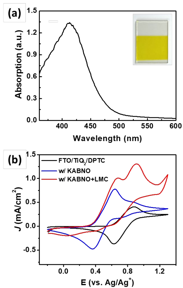
Figure 3. (a) UV-vis spectrum of FTO/TiO 2 /DPTC (inset: picture of a FTO/TiO 2 /DPTC electrode). (b) CVs of FTO/TiO 2 /DPTC (black), the same with 3 mM KABNO (blue), and the mixture of 3 mM KABNO and LMC (red) in 0.1 M TBAPF 6 acetonitrile.
