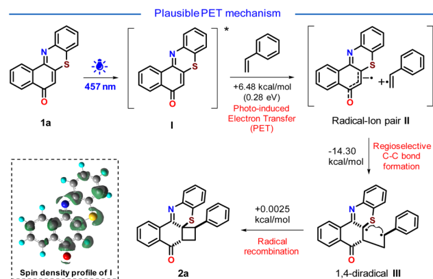
Scheme 5 Plausible reaction mechanism of the [2 + 2] photocycloaddition. The calculated relative Gibbs free energy of the reaction ( \Delta G^\circ in \text{kcal mol}^{-1} ) was obtained at a DFT-B3LYP/6-311+G(d,p)/CPCM(acetone) level of theory.
