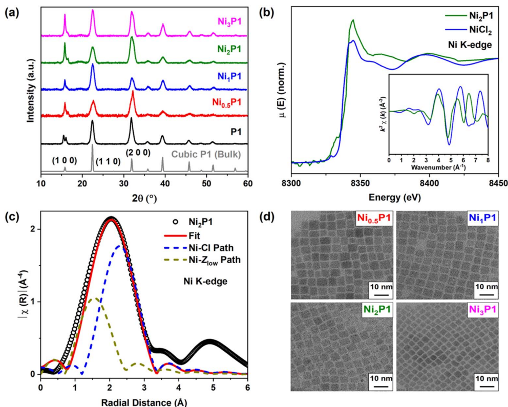
Fig. 1 Structural characterization: (a) XRD pattern of undoped (P1) and various Ni-doped CsPbCl 3 (Ni x P1; x = 0.5, 1, 2, 3) NCs with bulk cubic CsPbCl 3 data as reference (reference data obtained from inorganic crystal structure database) indicating the cubic ( Pm3m ) phase preserved upon doping. (b) Ni K-edge XANES spectra as a function of incident photoelectron energy along with inset of k 3 -weighted k -space spectra of Ni 2 P1 and NiCl 2 precursor, suggesting the oxidation state of Ni is +2. (c) k 3 -weighted magnitude of Fourier-transformed Ni K-edge EXAFS spectra of Ni 2 P1 (black hollow circle) and best fit (red solid line) along with the possible theoretical paths (dashed lines) for fitting. Dominant Ni–Cl interactions confirm the successful doping of Ni 2+ . (d) High-resolution TEM images of all Ni-doped CsPbCl 3 NCs showing monodisperse cubic NCs.
