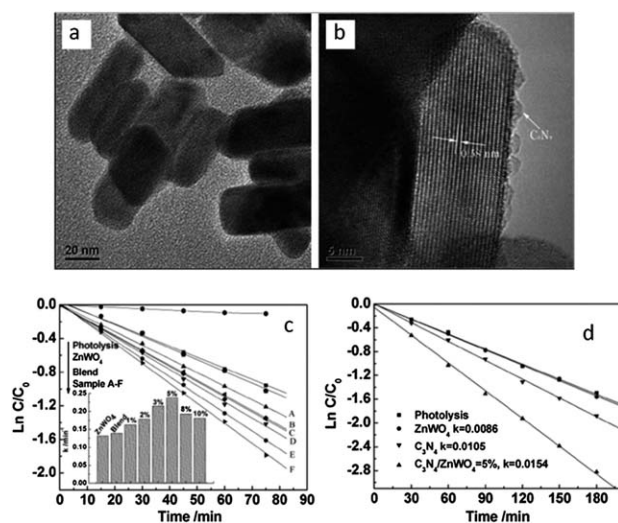
Fig. 13 The morphology of ZnWO_4 and C_3N_4 /ZnWO 4 photocatalysts: (a) ZnWO_4 (b) C_3N_4 /ZnWO 4 ; pseudo-first-order rates of MB degradation over ZnWO_4 and C_3N_4 /ZnWO 4 photocatalysts: (c) under UV light irradiation ( \lambda = 254 nm) (d) under visible light irradiation ( \lambda > 420 nm) (reprinted with permission from ref. 26, copyright 2012 Royal Society of Chemistry).
