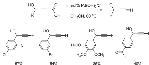
Scheme 53 Decarboxylation using Pd(OH) 2 /C.
