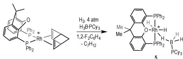
Scheme 8 Formation of complex 5. [\text{Bar}^{\text{F}}_4]^- anion not shown.
