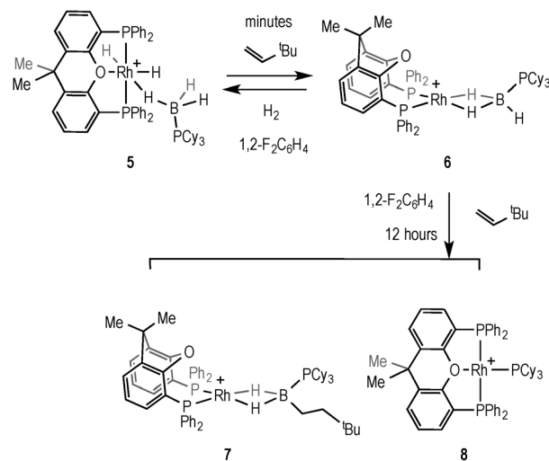
Scheme 9 Formation of 6 , 7 and 8 . [\text{BAr}^{\text{F}}_4]^- anions are not shown.
