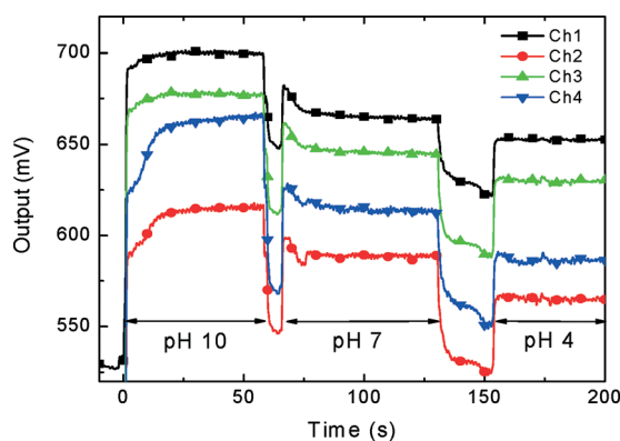
Fig. 10 Application of the 4 nanowire sensor to detect pH variations. 1 \mu\text{L} of buffer solution was manually dispensed for about 60 s and removed by capillary force before the new buffer was dispensed.
