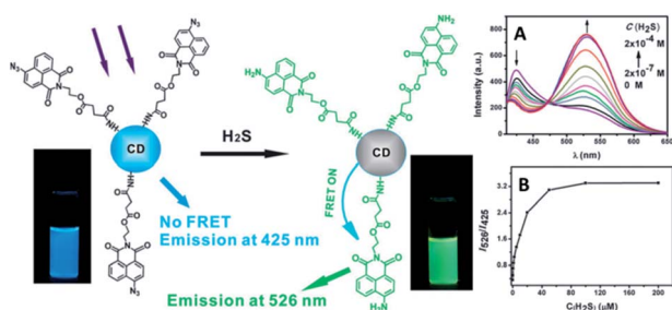
Fig. 31 (Left) Schematic illustration for the structure of the CQD-based sensor and its ratiometric detection of \text{H}_2\text{S} . Photographs were obtained under a hand-held UV lamp. (Right) (A) Fluorescence spectra of the CQD-based sensor (concentration: 0.45 \text{ mg mL}^{-1} ) in the presence of different amounts of \text{H}_2\text{S} ; (B) fluorescence intensity ratio of the CQD-based sensor as a function of \text{H}_2\text{S} concentration in HEPES buffered (pH 7.4) water–ethanol (3 : 1, v/v) ( \lambda_{\text{exc}} = 340 \text{ nm} ). Adapted with permission. 139 Copyright 2013, Royal Society of Chemistry.
