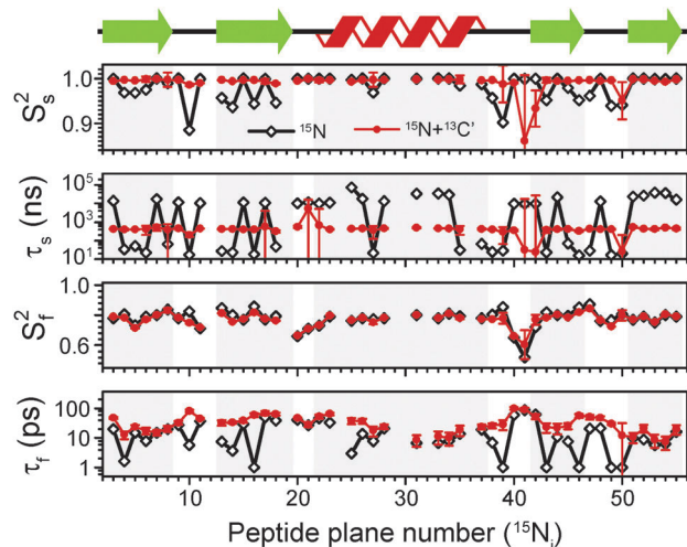
Fig. 5 Comparison of an extended model free (EMF) analysis of backbone dynamics based on ^{15}\text{N} R_1 and R_{1\rho} relaxation (black line) and combined ^{15}\text{N} R_1 and R_{1\rho} and ^{13}\text{C}' R_1 and R_{1\rho} relaxation for the sites in the same peptide planes (red line). S_s^2 , \tau_s , S_f^2 , \tau_f are, respectively: order parameter for the slow motion (reflecting amplitude of motion), correlation time for the slow motion, order parameter for the fast motion and correlation time for the fast motion. Measurements performed both at 600 and 850 MHz spectrometers were used in both cases. The overall amplitude of motion was constrained by measurements of NH dipolar couplings, which are averaged by motions faster than the inverse of its rigid limit value. The data for which NH dipolar couplings were not available or for which severe peak overlap hindered accurate measurement of relaxation rates were excluded.
