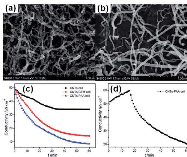
Fig. 28 SEM images of (a) CNTs and (b) CNTs-PAA composite electrodes; (c) electrodesorption process for the CNTs cell, CNTs-PAA cell and CNTs-CEM cell; (d) electrodesorption behavior for the CNTs-PAA cell under an applied voltage of -1.2 V. (Reproduced with permission from ref. 146.)
