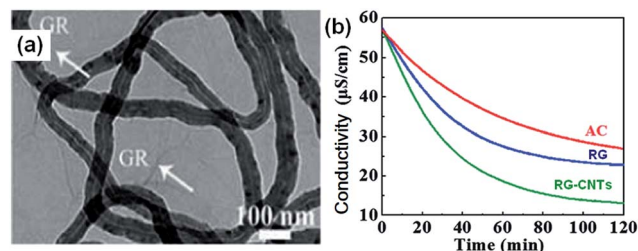
Fig. 10 (a) TEM image of the RG-CNTs composite with 10 wt% CNTs; (b) comparison of the CDI profiles for the RG-CNTs (10 wt% CNTs), RG and AC electrodes in an NaCl aqueous solution. (Reproduced with permission from ref. 84.)
