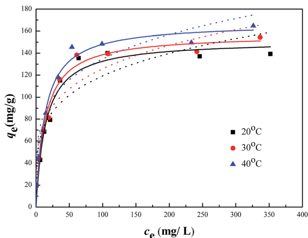
Fig. 9 Langmuir isotherm (solid line) and Freundlich isotherm (dash line) for the adsorption of Cr(vi) on CMB (reaction conditions: c_0 = 20\text{--}500 mg L ^{-1} ; V = 50 mL; m = 50 mg; t = 6 h; pH = 2; T = 20, 30, 40 °C).
