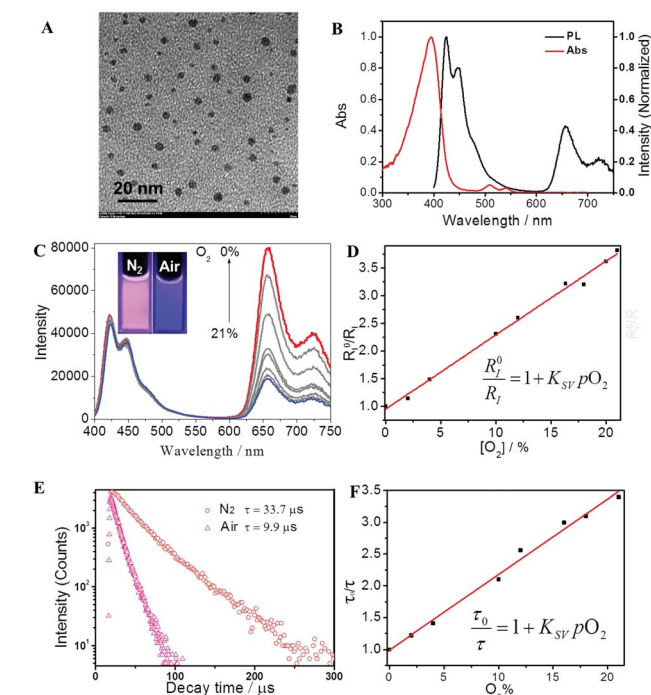
Fig. 2 (A) A TEM image of FP-Pdots in aqueous solution; (B) normalized absorption and emission spectra of FP-Pdots (12 \mu\text{g mL}^{-1} ) in aqueous solution; (C) emission spectra of FP-Pdots (12 \mu\text{g mL}^{-1} ) in H 2 O under the different O 2 concentrations; inset: the emission photos of FP-Pdots in the presence and absence of O 2 ; \lambda_{\text{ex}} = 375 nm. (D) Plot of R_0/R_1 as a function of O 2 concentration; (E) phosphorescence decays of FP-Pdots in aqueous solution saturated with N 2 or air, monitored at 656 nm from the Pt(II) porphyrin moiety; \lambda_{\text{ex}} = 405 nm. (F) Plot of \tau_0/\tau as a function of O 2 concentration ( \lambda_{\text{ex}} = 405 nm).
