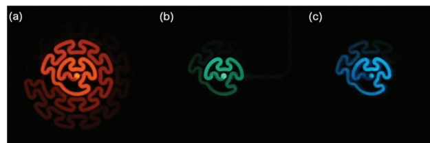
Fig. 4 Photographs of the chemiluminescence reactions of (a) [Ru(bpy) 3 ] 2+ and 1-(4-trifluoromethylphenyl)piperidin-4-ol, (b) [Ir(ppy-SO 3 ) 2 (pt-TEG)] - and 1-(4-trifluoromethylphenyl)piperazine, and (c) [Ir(df-ppy) 2 (pt-TEG)] + and furosemide, in aqueous solution. The metal complex reagents were continuously merged with an oxidant solution (cerium(IV) sulfate in 0.05 M H 2 SO 4 ) at a T-piece shortly prior to mixing with the other reactant solution within a transparent serpentine flow-cell. 22 A Canon 6D camera with 50 mm f1.8 lens were used (Canon, Japan). The exposure time and reactant concentrations were adjusted to produce similar emission intensities.
