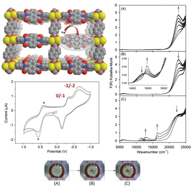
Fig. 2 Solid state electrochemistry and vis/NIR spectroelectrochemistry of [Zn 2 (ndc) 2 (DPNI)]. Cyclic voltammetry reveals two redox waves corresponding to generation of the radical anion and dianion states of the redox-active DPNI ligand. The optical properties of these states can be rapidly accessed using spectroelectrochemistry for generation of the radical anion (A) and dianion (B) states, which are accompanied by marked colour changes as seen in the photographs of the MOF on the transparent working electrode (bottom). Application of a more reducing potential leads to framework degradation (C). Reproduced from ref. 9 with permission from the Royal Society of Chemistry.
