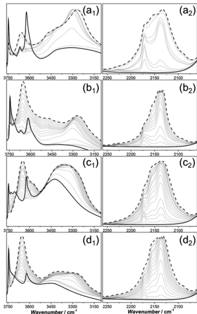
Fig. 4 FT-IR spectra measured at -130\text{ }^{\circ}\text{C} after adding increasing dosages of CO on (a) Sigma1-120-M; (b) ZSM-58; (c) Sigma1-315-S; (d) Sigma1-315-S-m. Panels a_1 , b_1 , c_1 and d_1 report the spectra in the hydroxyl group range ( 3760\text{--}3100\text{ cm}^{-1} ), while panels a_2 , b_2 , c_2 and d_2 report the CO vibrational mode region ( 2260\text{--}2060\text{ cm}^{-1} ). The bold solid line represents pretreated catalysts in vacuum, while the dashed black curves represent spectra collected at 30 mbar CO equilibrium.
