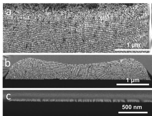
Fig. 4 Effect of the gold nanorod concentration on the internal organization. SEM images of internal sections of GNR supercrystals after FIB cutting. GNR concentrations were 375 mM (a), 37 mM (b) and 8.3 mM (c).
