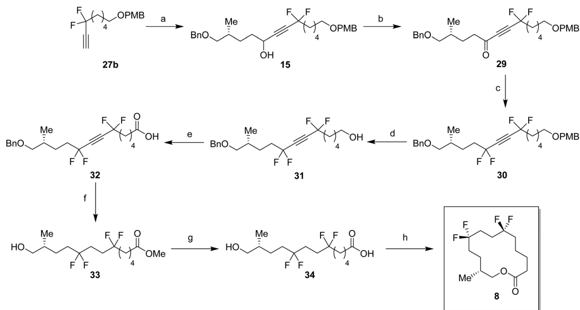
Scheme 4 Synthesis of musk lactone 8 . Reagents and conditions: (a) (i) n\text{BuLi} , THF, -78\text{ }^\circ\text{C} , 30 min. (ii) Aldehyde 12 , THF, -78\text{ }^\circ\text{C} –r.t., 20 h, 61%; (b) DMP, DCM, r.t., 2 h, 89%; (c) DAST, 50 °C, 18 h, 71%; (d) DDQ, DCM, \text{H}_2\text{O} , r.t., 2 h, 78%; (e) BAIB, TEMPO, \text{CH}_3\text{CN} , \text{H}_2\text{O} , r.t., 7 h, 58%; (f) palladium on carbon (10 wt%), \text{H}_2 , MeOH, r.t., 18 h, 65%; (g) LiOH, THF, \text{H}_2\text{O} , r.t., 3 h, 94%; (h) 2,4,6-trichlorobenzoyl chloride, \text{NEt}_3 , THF, r.t., 2.5 h. (ii) 4-DMAP, toluene, r.t., 3.5 h, 54%.
