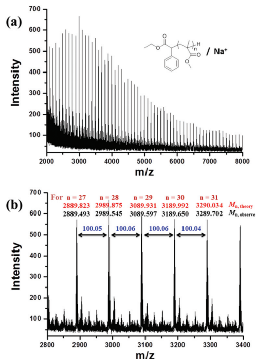
Fig. 6 (a) MALDI-TOF mass spectrometry results in the round mode of PMMA ( M_{n, GPC} = 13\,800\text{ g mol}^{-1} , M_w/M_n = 1.53 ) obtained by metal-free ATRP of MMA with fluorescein (FL) as an organic photocatalyst. (b) Enlargement of the MALDI-TOF-MS of PMMA from m/z 2800 to 3400.
