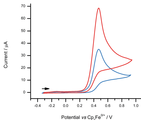
Fig. 4 CVs comparing the electrochemical behaviour of 1\text{-H} (1.8 mM) with (red line) and without (blue line) the addition of excess Brønsted base (2,6-lutidine; 6.7 mM) at a scan rate of 100 \text{ mV s}^{-1} .
