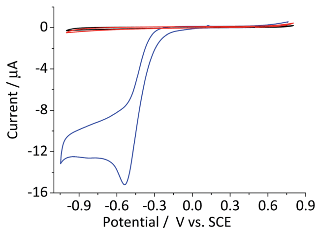
Fig. 3 Cyclic voltammetric curves of a bare glassy carbon electrode (red) and that modified with 2.4 \times 10^{-5} \text{ g cm}^{-2} of hematite nanoparticles in \text{N}_2 saturated 20 mM KCl with 1.5 mM \text{H}_2\text{O}_2 collected at the scan rate of 0.01 \text{ V s}^{-1} . Black line illustrates a cyclic voltammetric curve of bare glassy carbon in the same KCl solution without \text{H}_2\text{O}_2 .
