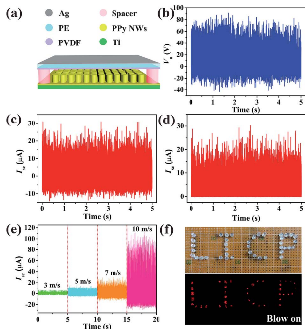
Fig. 5 (a) Device structure of the designed PPy NW-based W-TENG. (b) V_o , (c) I_{sc} and (d) the rectified I_{sc} at a wind speed of 7 \text{ m s}^{-1} (on the scale of 4 BF). (e) The I_{sc} at different wind speeds from 3 \text{ m s}^{-1} (2 BF) to 10 \text{ m s}^{-1} (5 BF). (f) Photographs of 40 LEDs before and after being powered by the W-TENG.
