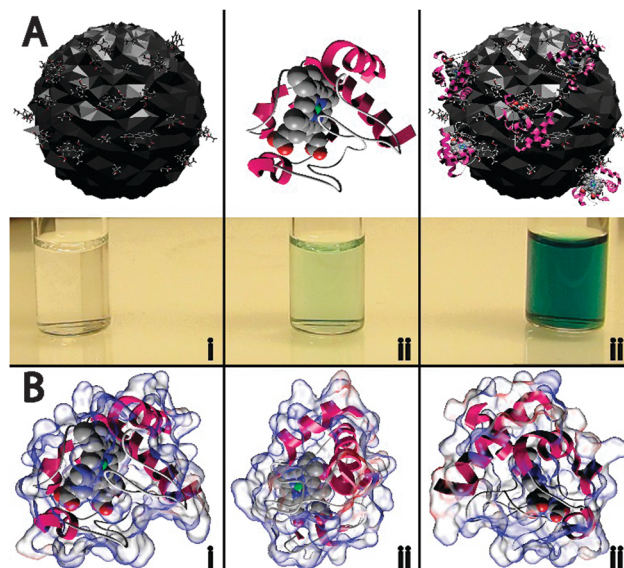
Fig. 1 (A) Neat carbon nanodots (C-dots) did not display any catalytic activity, as evidenced by the lack of green color in (Ai), while native cytochrome c (cyt c) was found to exhibit weak peroxidase activity (Aii). When C-dots were combined with cyt c, the peroxidase activity was dramatically enhanced, indicated by the rapid formation of the oxidized form of ABTS ( i.e. , appearance of intense green color), as shown in (Aiii). (B) Different orientations of the electrostatic calculations performed on cyt c show that a majority of the protein surface is positively charged (blue areas), with the bulk of the positive charge residing in the vicinity of the heme group.
