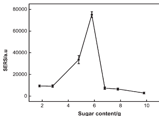
Fig. 2 SERS performance of Ag NPs-modified PDMS sponge prepared with varying amounts of sugar. A total of 10 \mu L of R6G (1 \mu M) was used as the Raman probe. Laser power: 14 mW. Integration time: 2 s. Objective: 20 \times .
