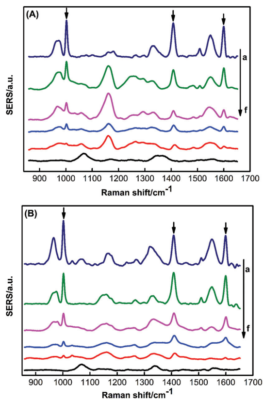
Fig. 6 SERS spectra of triazophos from the surface of cherry tomatoes (A) and plum (B). The concentrations of triazophos were: (a–f) 10 \mu\text{L} 50 ppm, 10 ppm, 5 ppm, 1 ppm, 0.1 ppm, 0 ppm, respectively. Laser power: 10 mW. Integration time: 50 s. Objective: 20 \times .
