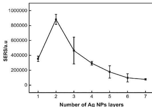
Fig. 3 SERS performance of different Ag NPs rounds-modified PDMS sponge. 10 \mu L R6G (1 \mu M) was used as the Raman probe. Laser power: 14 mW. Integration time: 2 s. Objective: 20 \times .
