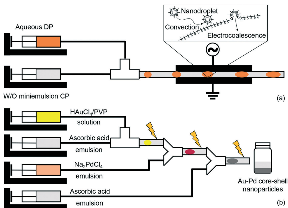
Fig. 1 (a) Experimental setup for generating aqueous microdroplets with a W/O miniemulsion and electrocoalescence. (b) Three electrocoalescence-assisted chemical addition steps for Au-Pd core-shell nanoparticle synthesis.
