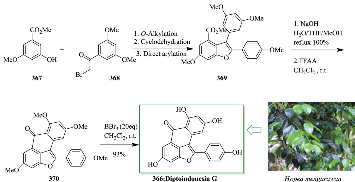
Scheme 77 Total synthesis of diptoindonesin G 366 .
