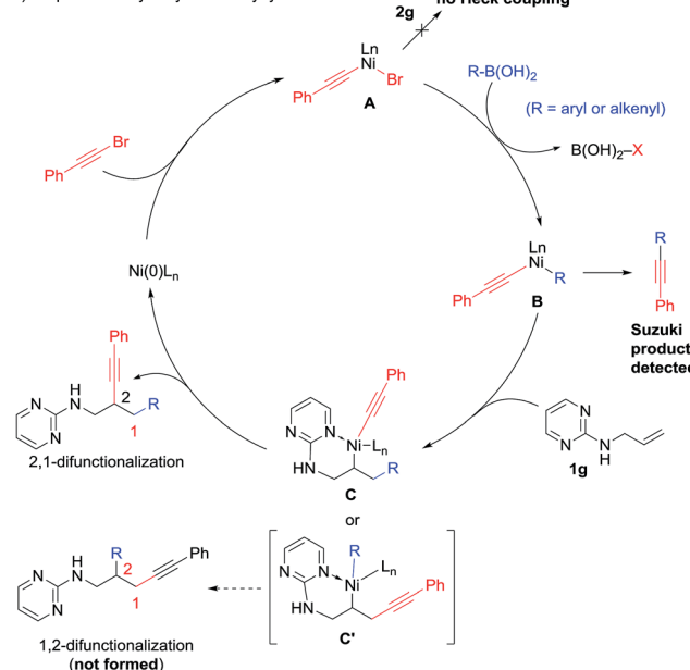
Scheme 8 Proposed mechanism for alkynylarylation.
