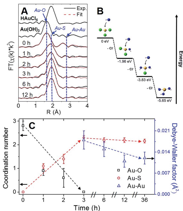
Fig. 5 (A) Au L_3 -edge FT-EXAFS with fitted spectra and reference materials. (B) Relative DFT energies of \text{AuCl}_3 (set to 0 eV), \text{Au}(\text{OH})_3 , and intermediate products of the precursor ion-exchange process. (C) Coordination and Debye-Waller (Au-Au shell only) plot for time-dependent EXAFS fitting results.
