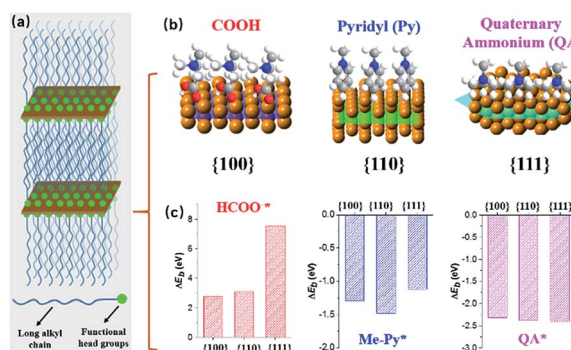
Fig. 1 Schematic illustration for surface facet-controlled synthesis of ultrathin PdNs. (a) Scheme to show the assembled lamellar meso-phases between long-chain alkyl surfactants and the growth of Pd nanocrystals. (b) Surface binding behaviours and (c) corresponded \Delta E_b of functional head groups onto different Pd crystal planes based on first-principles calculations.
