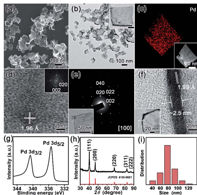
Fig. 2 Structural characterizations of ultrathin 2D PdNSs{100} synthesized using C_{22}N-COOH(Br^-) . (a) Low-magnification SEM and (b) TEM images of PdNSs{100}. Inserted in (b) is TEM image of an individual PdNS and the scale bar is 20 nm. (c) STEM image and elemental mapping of PdNSs{100}. (d) HRTEM image and corresponded FT pattern of PdNSs{100}. (e) SAED pattern of an individual PdNSs{100} (shown in the inset). (f) HRTEM image taken from the curly edge of a PdNS (the insert) which stands vertically on the TEM grid. (g) Pd 3d XPS spectrum, and (h) wide-angle XRD pattern of PdNSs{100}. (i) The average size and its distribution of PdNSs{100}.
