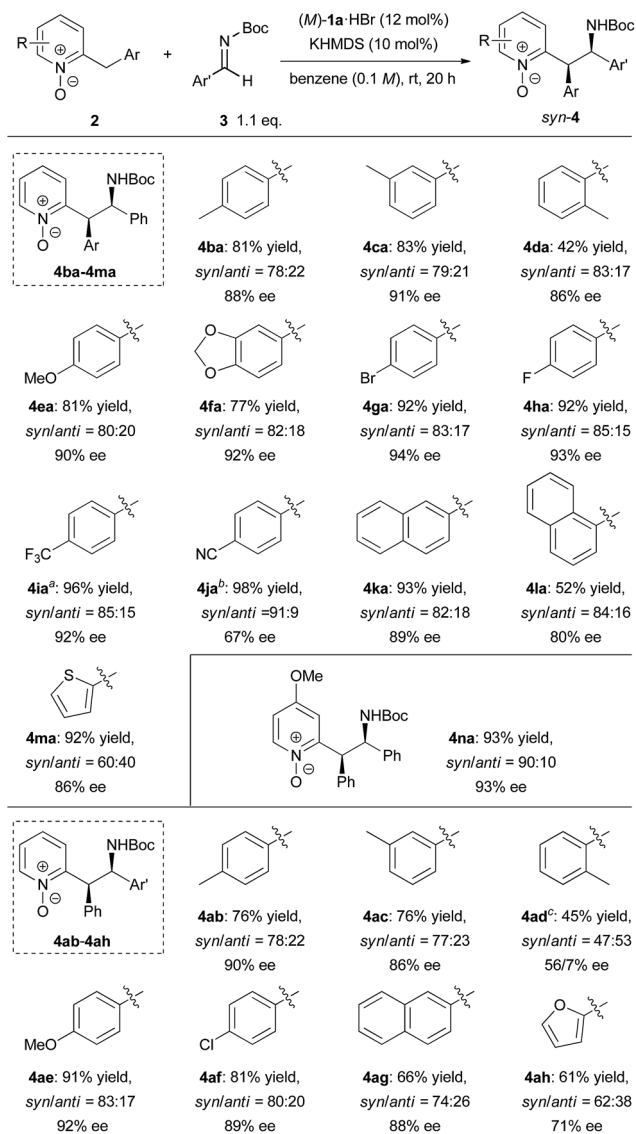
Scheme 2 Substrate scope. Unless stated otherwise, the reaction conditions were as follows: 2 (0.10 mmol), 3 (0.11 mmol), (M) - 1a ·HBr (0.012 mmol), KHMDS (0.010 mmol), benzene (1.0 mL), rt, 20 h. The combined yield of the diastereomeric mixtures is indicated. The dr and ee values were determined by chiral stationary phase HPLC analysis. The ee values of the major isomers are indicated. a The reaction was conducted in toluene at 0 °C and the concentration was 0.025 M. b The reaction was conducted in toluene at −30 °C for 4 h. c The absolute configuration was not confirmed. The minor and major isomers were obtained with 56% ee and 7% ee, respectively.
