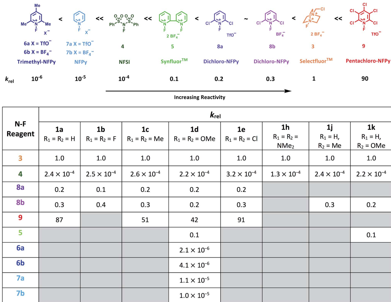
Fig. 5 Quantitative reactivity scale of N-F fluorinating reagents. Relative rate constants were calculated based on the absolute rate constants shown in Table 1, with Selectfluor TM 3 as the reference electrophile.
