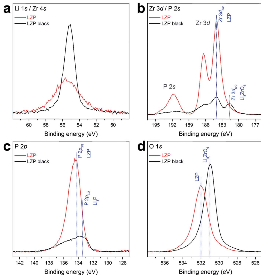
Fig. 7 XPS core levels of L郑-1100 and the black surface layer (L郑 black) formed after cycling a Li/L郑/Li cell at 80^\circ\text{C} for 100 h, including (a) Li 1s/Zr 4s, (b) Zr 3d/P 2s, (c) P 2p, and (d) O 1s.
