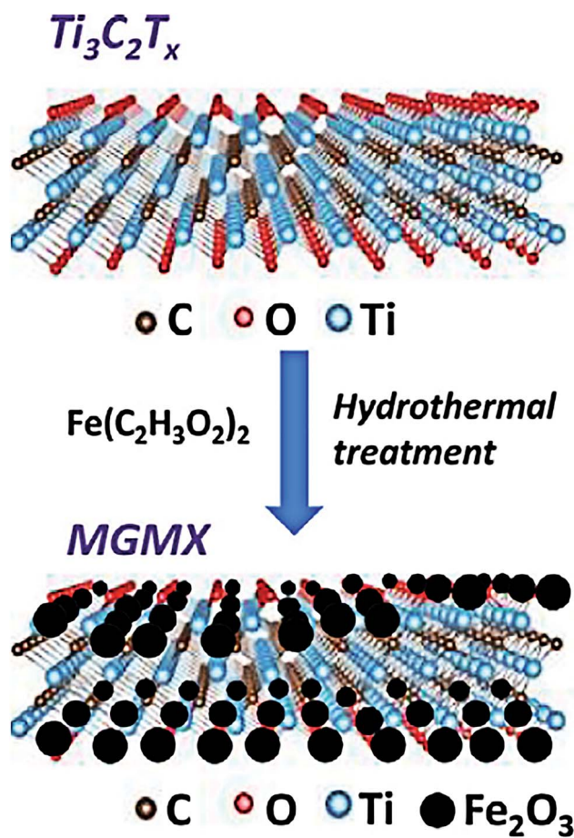
Fig. 8 Schematic structure of the composite formed by MXenes and Fe_2O_3 . 22 This figure has been adapted from ref. 22 with permission from Elsevier.
