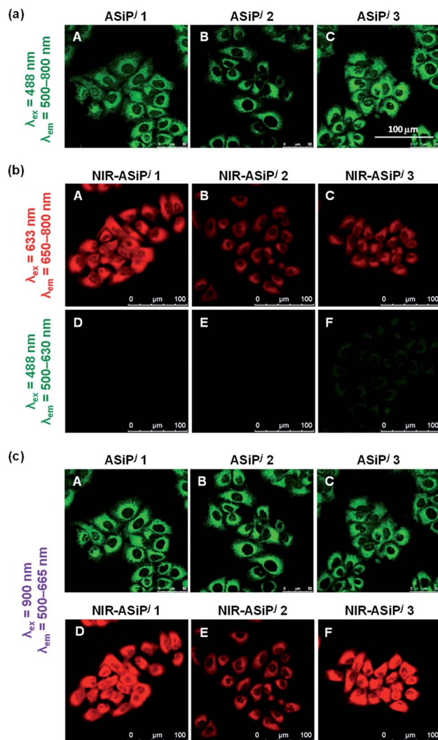
Fig. 4 (a) CLSM images of A549 cells incubated with ASiP d dyes ( 1.0 \mu\text{M} ) for 30 min. The images were obtained by excitation at 488 nm and collection of the emissions in the range of 500–800 nm. (b) CLSM images of A549 cells incubated with NIR-ASiP d dyes ( 10 \mu\text{M} ) for 30 min. The images were obtained by collecting emissions either from (A–C) the NIR channel (650–800 nm) under excitation at 633 nm or from (D–F) the green channel (500–630 nm) under excitation at 488 nm. (c) TPM images of ASiP d (A–C) and NIR-ASiP d (D–F) dyes. The images were obtained by excitation at 900 nm and collection of the emissions in the range of 500–665 nm. Scale bar: 100 \mu\text{m} .
