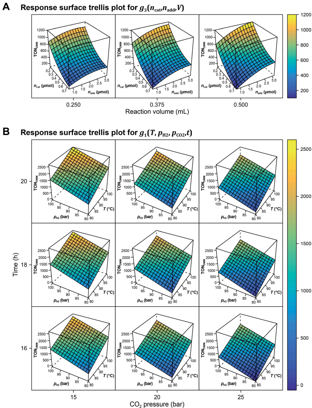
Fig. 3 Calculated response surfaces. (A) Trellis plot of the response surface for g_3(n_{\text{cat}}, n_{\text{add}}, V) from OLS modelling with T = 90^\circ\text{C} , p_{\text{H}_2} = 90 bar, p_{\text{CO}_2} = 20 bar and t = 18 h. (B) Response surface trellis plot of the linear OLS model for g_1(T, p_{\text{H}_2}, p_{\text{CO}_2}, t) with n_{\text{cat}}^* = 0.075 \mu\text{mol} , n_{\text{add}}^* = 3.576 \mu\text{mol} and V^* = 0.550 mL. For a mathematical definition of the polynomial parametric surrogates, g_{1,3}() , see the Methods section.
