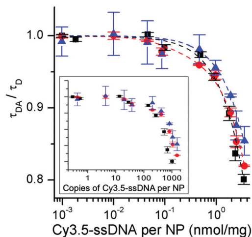
Fig. 6 Cy3.5-ssDNA concentration dependent PL decay time ratios of quenched ( \tau_{\text{DA}} ) and unquenched ( \tau_{\text{D}} – no Cy3.5-ssDNA) c-UCNPs (black) and css-UCNPs (red) upon excitation at 980 nm and of css-UCNPs upon 808 nm excitation (blue). Inset shows the same ratios as a function of amount (copies) of Cy3.5-ssDNA per NP.
