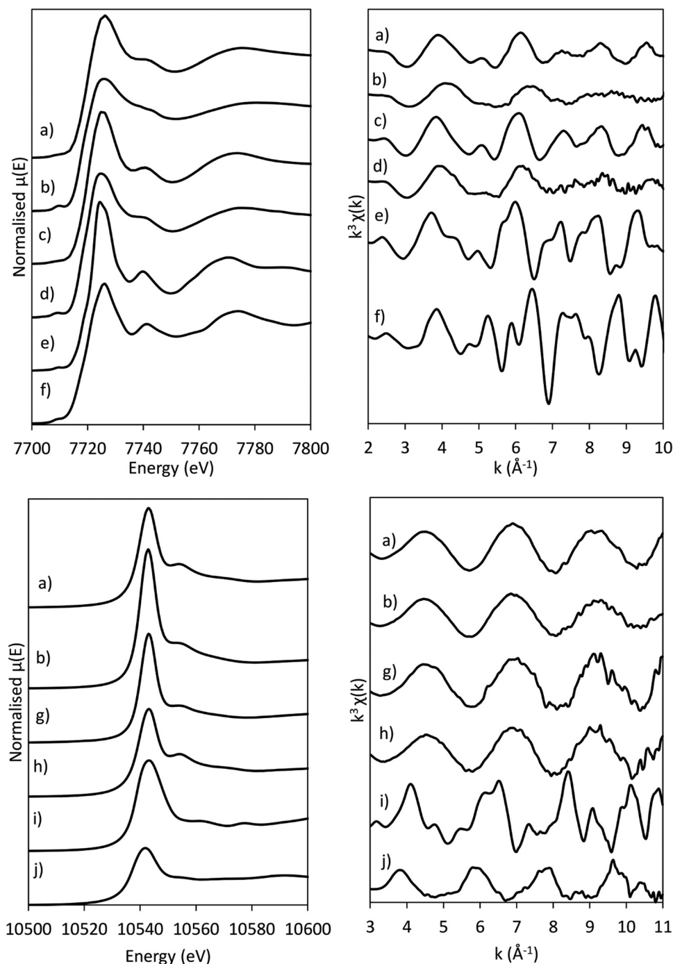
Fig. 4 XANES spectra (left) and k^3 -weighted \chi -curves (right) of the (a) as-synthesised CoRe-gel, (b) annealed CoRe-gel, (c) as-synthesised Co-gel, (d) annealed Co-gel, (e) \text{Co(OH)}_2 , (f) \text{CoO} , (g) annealed Re-gel, (h) \text{NH}_4\text{ReO}_4 , (i) \text{ReO}_3 and (j) \text{ReO}_2 at the Co K-edge (top) and at the Re L_{\text{III}} -edge (bottom).
