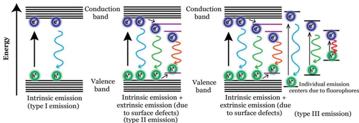
Fig. 4 Schematic representation corresponding to the emission mechanism in Cdot systems.
