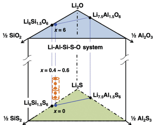
Fig. 1 Schematic composition diagram of the Li-Al-Si-S-O system (found between the pseudo-ternary \text{Li}_2\text{O}-\text{SiO}_2-\text{Al}_2\text{O}_3 and \text{Li}_2\text{S}-\text{SiS}_2-\text{Al}_2\text{S}_3 diagrams). The argyrodite-type phase appears in a narrow region, as indicated by a dashed cylinder. Samples with the \text{Li}_{6.15}\text{Al}_{0.15}\text{Si}_{1.35}\text{S}_{6-x}\text{O}_x (LASSO) ( 0.4 \leq x \leq 0.9 ) composition were synthesized.
