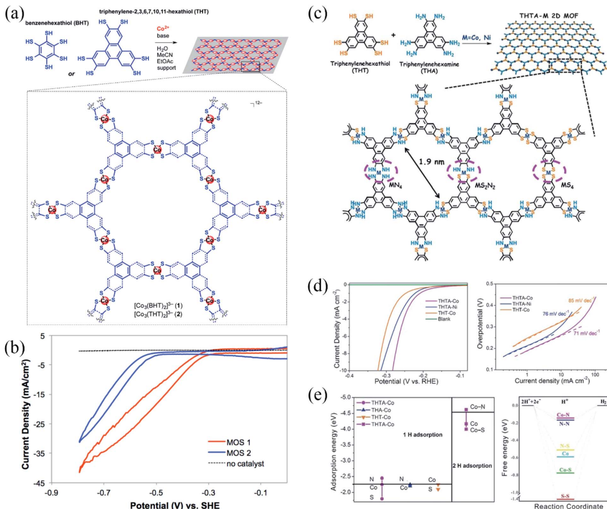
Fig. 18 (a) Synthesis of cobalt dithiolenes films, Co-BHT and Co-THT, the films are deposited onto the desired supports, generating \text{MOS}_1 and \text{MOS}_2 ; (b) polarization curves of \text{MOS}_1 (red) and \text{MOS}_2 (blue) at pH 1.3, scan rate, 100 \text{ mV s}^{-1} ; reproduced with permission. 162 Copyright©2015 American Chemical Society. (c) The synthesis of single-layer 2D MOFs, in which \text{MS}_2\text{N}_2 complexes along with \text{MN}_4 and \text{MS}_4 moieties were incorporated into the hexagonal networks through metal dithiolenes–diamine coordination (THTAM) ( \text{M} = \text{Co} and \text{Ni} ); (d) HER polarization plots (left) of three types of 2D MOFs: THTA-Co (purple), THTA-Ni (blue), and THT-Co (yellow) and a blank glassy carbon disk electrode in 0.5 \text{ M H}_2\text{SO}_4 and the Tafel plots (right) obtained from the polarization curves; (e) the adsorption energy of one H and two H radicals bonding to the proposed active sites on the surface of THTA-Co, THA-Co, and THT-Co 2D MOFs (left) and the free-energy diagram of the HER at the equilibrium potential for the THTA-Co 2D MOFs with the possible active sites (right). Reproduced with permission. 144 Copyright©2017 WILEY-VCH Verlag GmbH & Co. KGaA.
