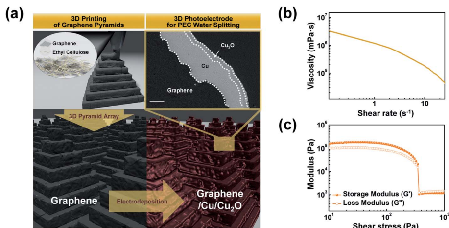
Fig. 1 (a) Schematic illustration of the fabrication process of 3D-printed photoelectrodes for water splitting via two successive steps: 3D printing of a pyramid array using graphene ink and functionalization via electrodeposition (Cu and \text{Cu}_2\text{O} layers). Scale bar is 20\ \mu\text{m} . (b) Viscosity vs. shear rate and (c) storage ( G' ) and loss ( G'' ) moduli vs. ink shear stress. During the printing process, the graphene ink transitions from a solid-like fluid to a liquid-like fluid as a function of the shear stress.
