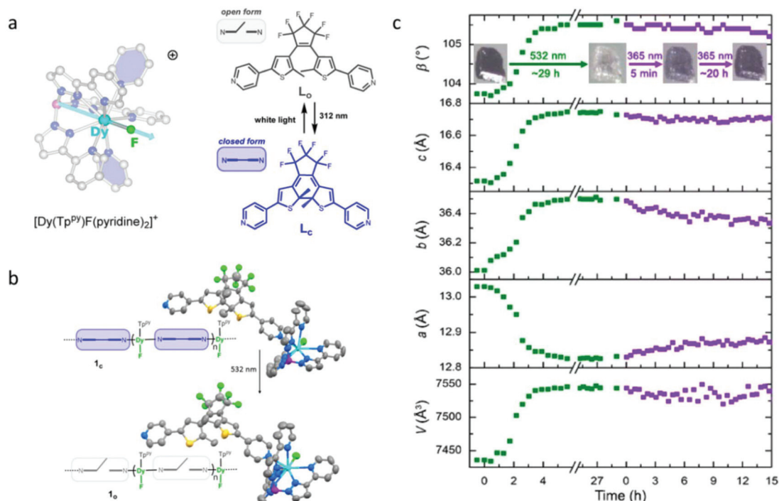
Fig. 1 (a) Molecular structure of [Dy(Tp Py )(pyridine) 2 ] + PF 6 - in the cationic form and the open and closed form of the photoactive bispyridyl dithienylethene unit used in building 1c; (b) single crystal structures of 1c and 1o; (c) evolution of the unit cell parameters of 1c upon continuous irradiation with 532 nm light (green dots) followed by 365 nm light (purple dots). Reproduced with permission from ref. 49. Copyright 2020 American Chemical Society. 49
