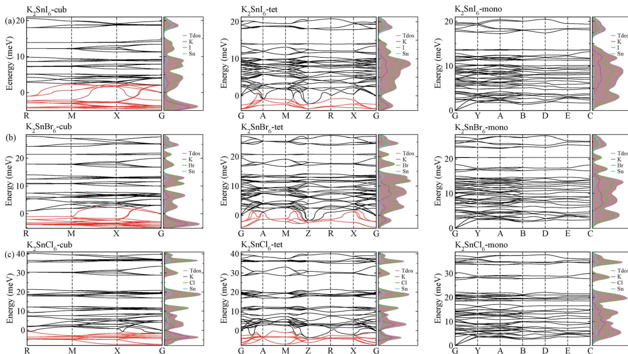
Fig. 4 Phonon dispersion curves and atomic resolved density of states in (a) \text{K}_2\text{SnI}_6 , (b) \text{K}_2\text{SnBr}_6 and (c) \text{K}_2\text{SnCl}_6 in the cubic (left), tetragonal (middle) and monoclinic (right) phases. Red lines show the anharmonic phonon modes with negative phonon energies.
