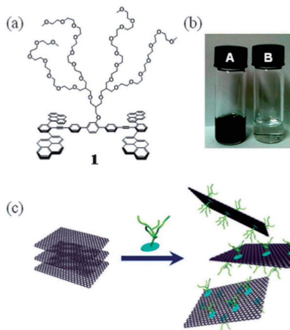
Fig. 13 Exfoliation process of graphite and stabilization of graphene through the \pi - \pi interaction with tetraterpene derivative. This figure has been reproduced from ref. 91 with permission from R. Soc. Chem. , Copyright 2016.
