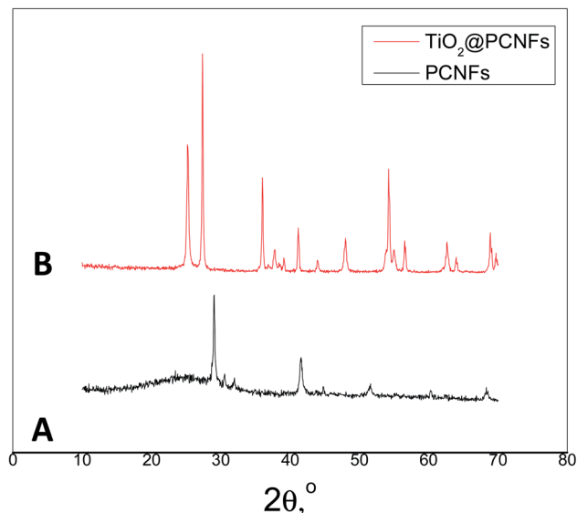
Fig. 3 XRD patterns of PCNFs (A), \text{TiO}_2 @PCNFs (B).
