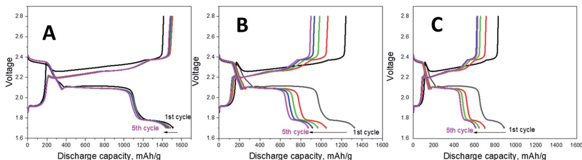
Fig. 5 Galvanostatic charge/discharge profiles of Li-S cells with \text{TiO}_2 @PCNF interlayer (A), PCNF interlayer (B) and without interlayer (C).
