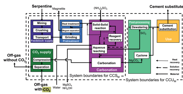
Fig. 6 Process flow diagram of carbon capture and utilization by mineralization via indirect concept of the Abo Academy pathway (AA pathway) using serpentine. Carbonation takes place in a fluidized bed (FB). \text{CCS}_M is carbon capture and storage by mineralization. \text{CCU}_M is carbon capture and utilization by mineralization.
